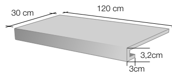
GRADINO LINEARE COSTA RETTA 30x120x3,2x3 - 12"x48"x1.2"x1"
