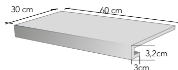
GRADINO LINEARE COSTA RETTA 30x60x3,2x3 - 12"x24"x1.2"x1"
